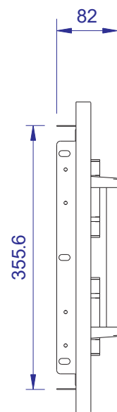
Side View
