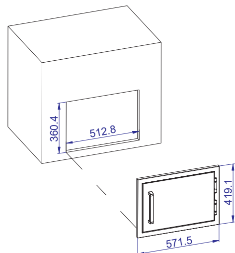
Cutout Size
