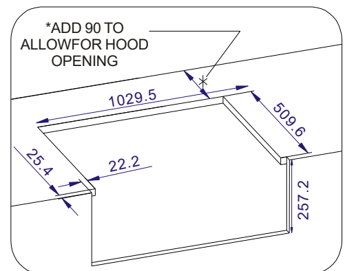
Cutout Size
